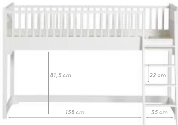
021213 Classic low loft bed 90 × 200 cm w 97 × l 207 × h 131 cm
